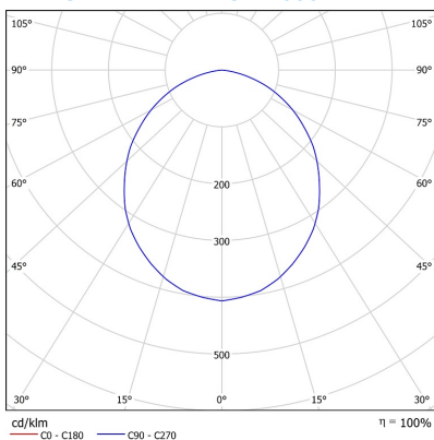
NECTRA LED IP44 25W 4000K WHITE
