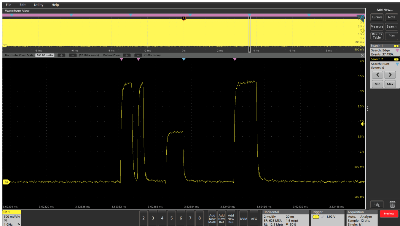
Figure 21: Earlier, FastAcq revealed the presence of a runt pulse in a digital data stream prompting further investigation. In this long 20 ms acquisition, Search 1 reveals that there are approximately 37,500 rising edges in the acquisition. Search 2 (run simultaneously) reveals that there are six runt pulses in the acquisition.
