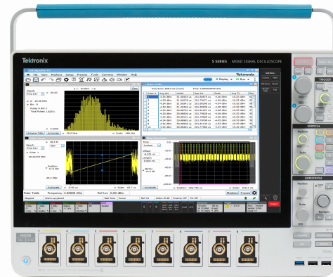
Figure 28: Pulse analysis on SignalVu-PC running on a 5 Series
