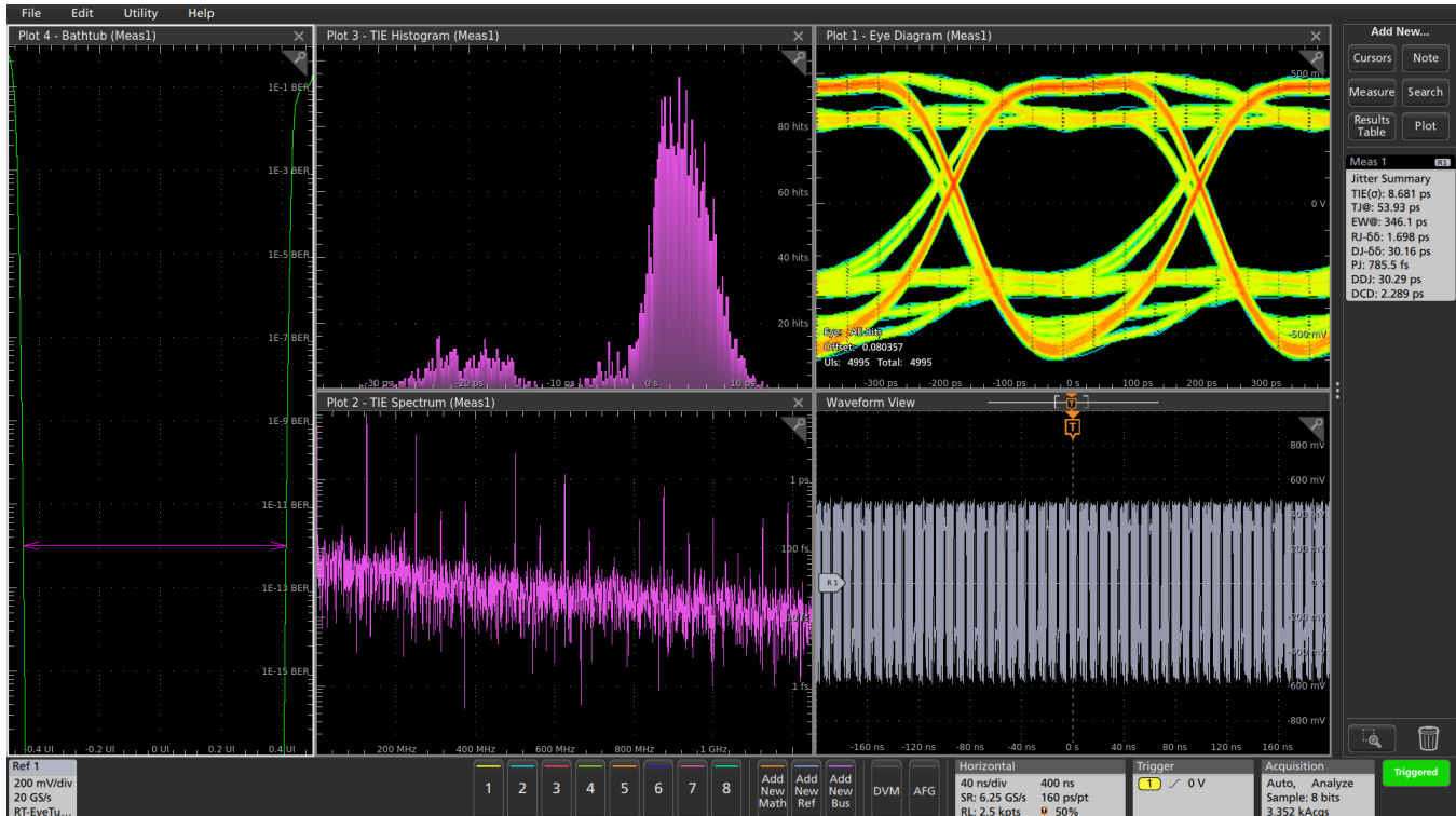
Figure 29: The unique Jitter Summary provides a comprehensive view of your device's performance in a matter of seconds.
