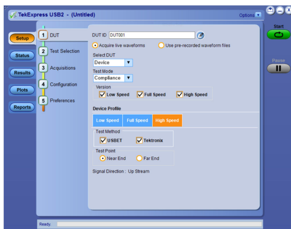
Figure 24: The TekExpress USB 2.0 automated compliance testing configuration menu.
