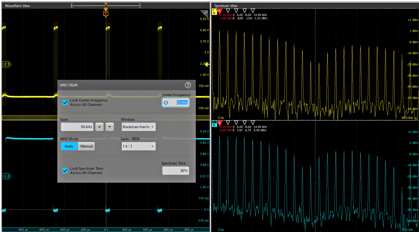
Figure 25: Intuitive spectrum analyzer controls like center frequency, span and resolution bandwidth (RBW), independent from time domain controls, provide easy setup for frequency domain analysis. A spectrum view is available for each FlexChannel analog input, enabling multi-channel mixed domain analysis.
