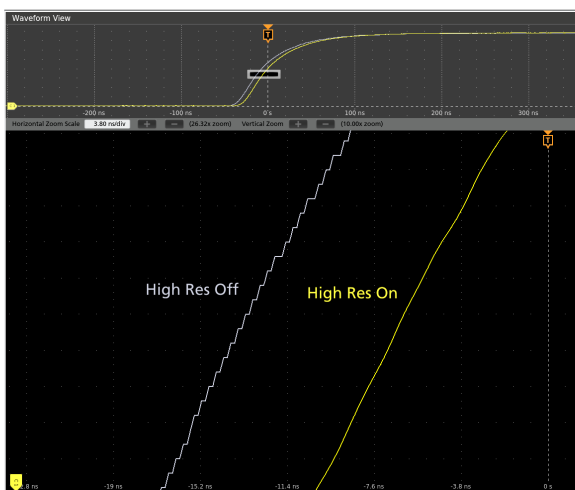
Figure 13: The 5 Series MSO's 12-bit ADC, along with the new High Res mode, enable industry leading vertical resolution.
