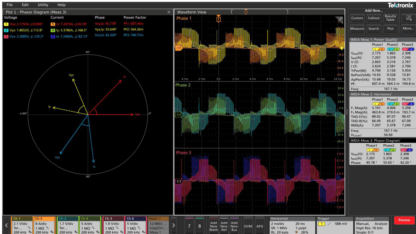
Figure 31: On the left is a Phasor Diagram displaying the phase and magnitude of current and voltage measurements for all three phases of power. In the results badge on the right, are the results from the automated measurements of power quality, power harmonics and the phasor diagram.
