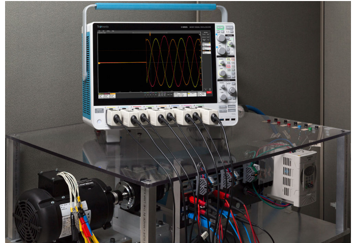
Figure 1: Voltage measurements on a three-phase motor showing the three-phase input voltages after start-up.
