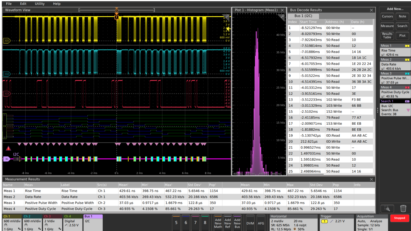
Figure 7: Viewing three analog channels, eight digital channels, a decoded serial bus waveform, decoded serial packet results table, four measurements, a measurement histogram, measurements results table with statistics and a search on serial bus events - simultaneously!
