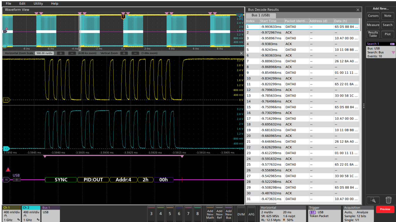
Figure 23: Triggering on a USB full-speed serial bus. A bus waveform provides time-correlated decoded packet content including Start, Sync, PID, Address, End Point, CRC, Data values, and Stop, while the bus decode table presents all packet content from the entire acquisition.
