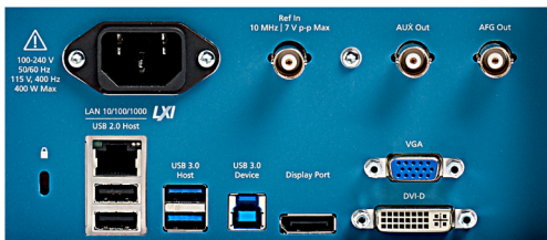
Figure 32: The I/O you need to connect the 5 Series MSO to the rest of your design environment.
