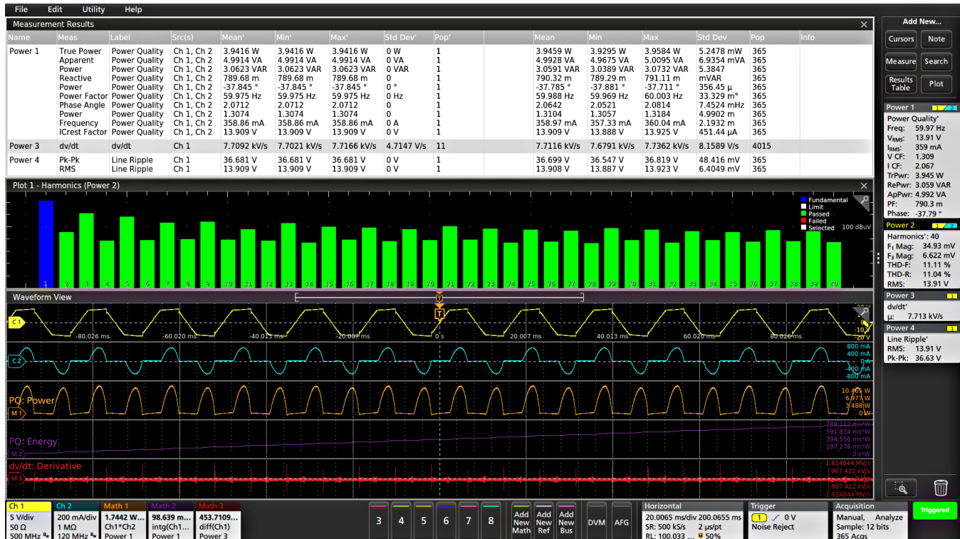
Figure 30: The Power Analysis measurements display a variety of waveforms and plots.
