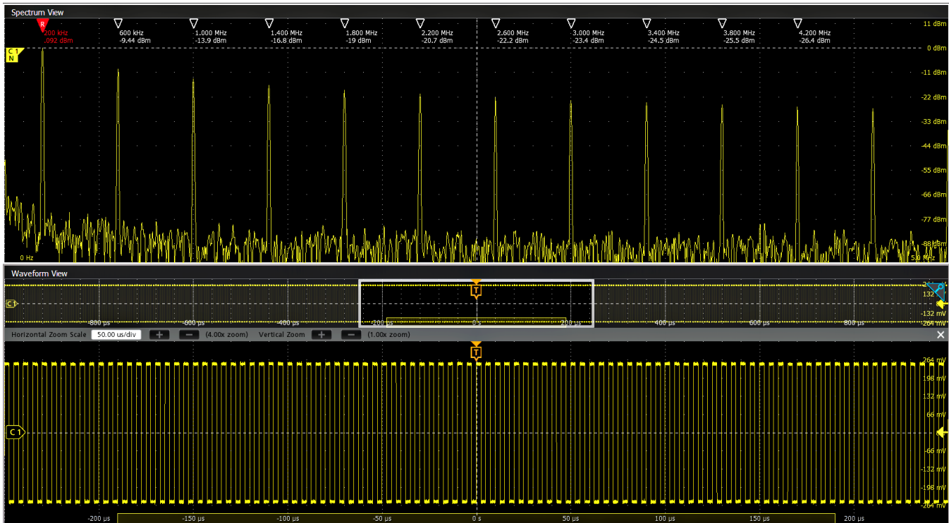
Figure 26: Spectrum Time gates the range of time where the FFT is being calculated. Represented by a small graphical rectangle in the time domain view, it can be positioned to provide time correlation with the time domain waveform. Perfect for conducting Mixed Domain Analysis. Up to 11 automated peak markers provide frequency and magnitude values of each peak. The Reference marker is always the highest peak shown and is indicated in red.
