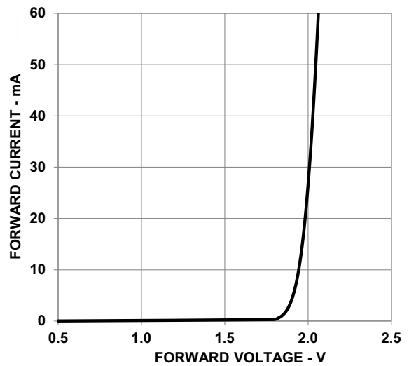
Figure 10: Forward Current vs. Forward Voltage
