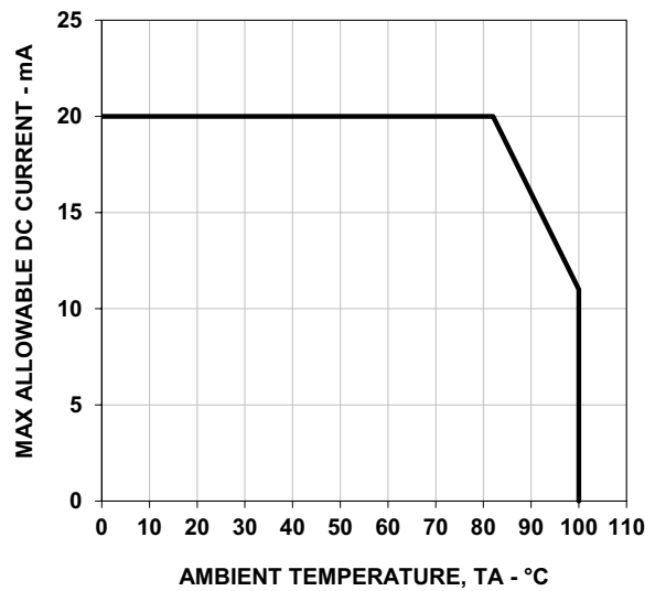
Figure 12: Maximum Forward Current vs. Ambient Temperature
