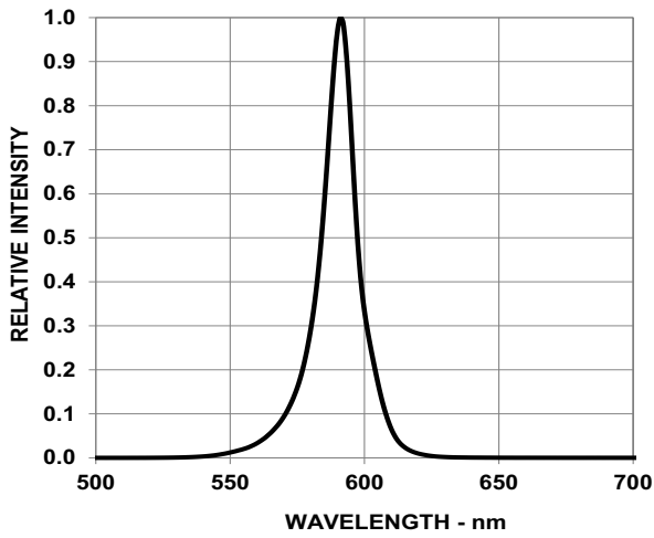
Figure 9: Relative Intensity vs. Wavelength
